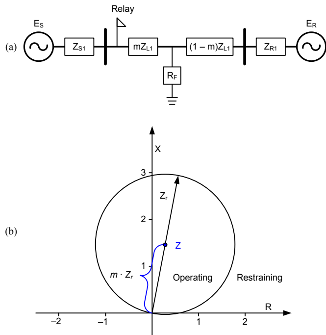
Fig. 1 Line fault at 50 percent of reach ( m = 0.5 p.u.): (a) System one-line diagram, (b) Mho characteristic.
